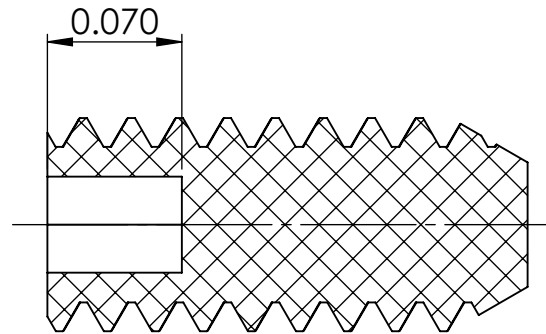
SECTION X-X
